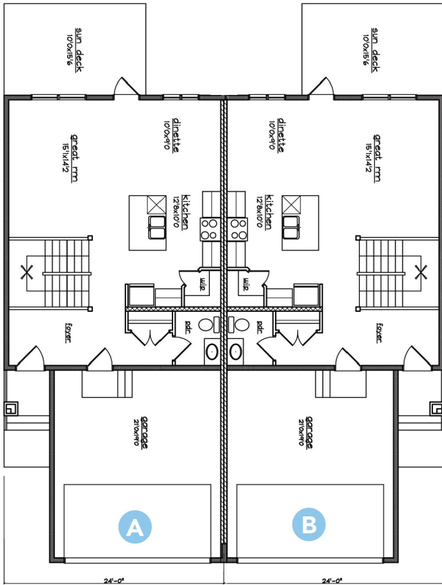
MAIN FLOOR
